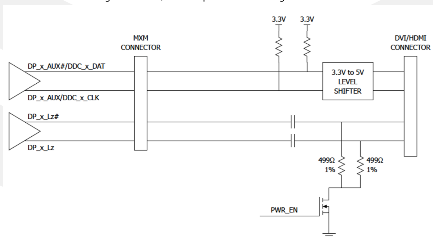
Figure 11.1 DVI/HDMI Implementation Using DP Interface
