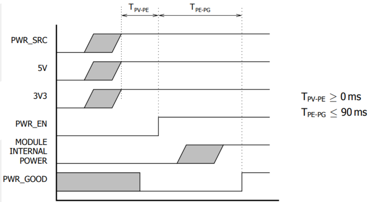
Figure 7.1 Power Sequencing
