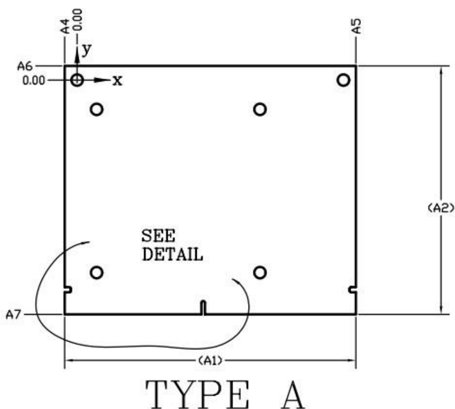
Figure 3.1: Board Outlines
