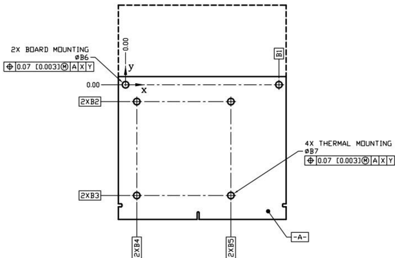
Figure 4.1 Mounting Holes
