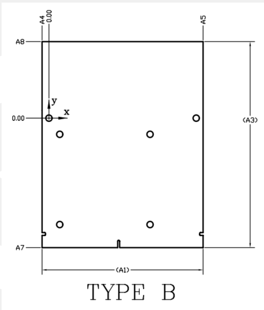
Figure 3.1 Board Outlines
